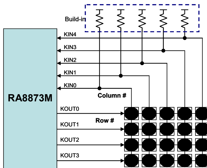
Figure 8-3 : Key-Pad Application
