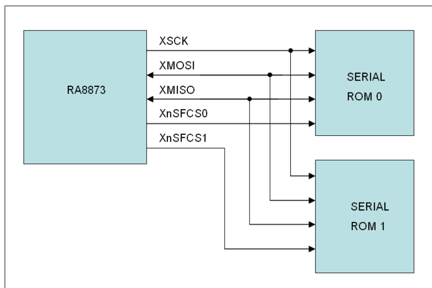
Figure 3.3: RA8873M Serial Flash/ROM System
